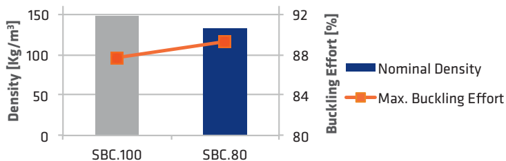
Fig. 2: Global buckling analysis of wind energy rotor blade.
